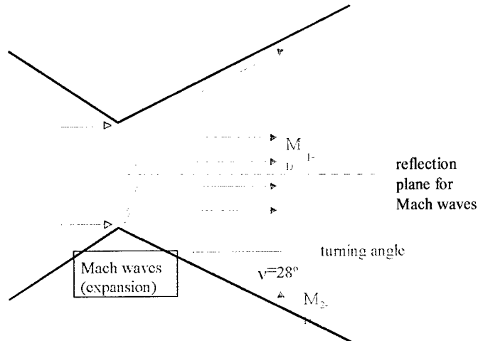
Figure 21. Nozzle Mach Expansion Waves
